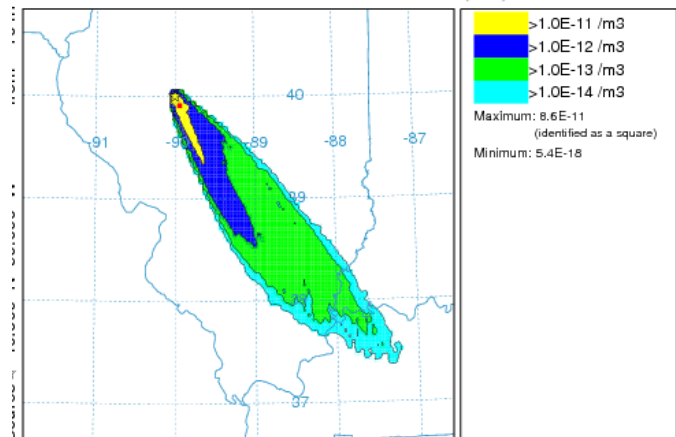
NOAA HYSPLIT MODEL Concentration (/m3) averaged between 0 m and 100 m Integrated from 0000 16 Oct to 1200 16 Oct 95 (UTC) TEST Release started at 0000 16 Oct 95 (UTC)
