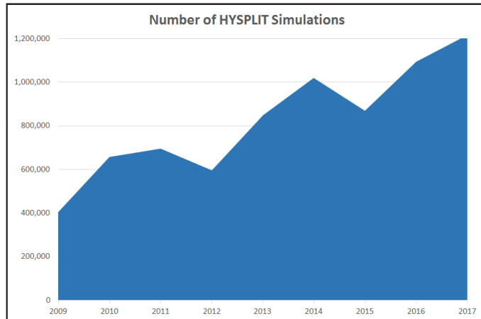
HYSPLIT simulations have seen a steady increase since usage tabulations began in 2009.
