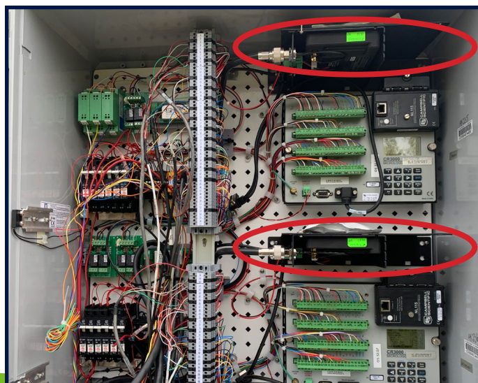
New transmitters inside the data logger box. Credit: Chuck Lindsay (Williwaw Weather and Climate Services)
