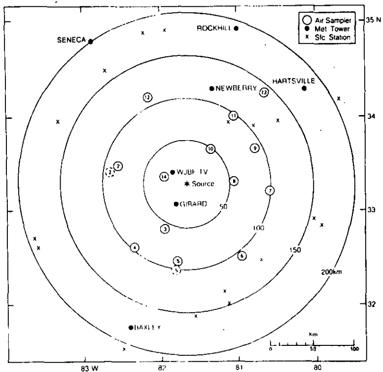
FIGURE 1. Krypton-85 Cryogenic Air Sampling Stations, Meteorological Towers and Surface Weather Stations Within 200 km of the SRP Source. Dashed circles indicate earlier sampling location.
