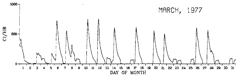
FIGURE 2j. Krypton-85 Release Rate for February and March, 1977
