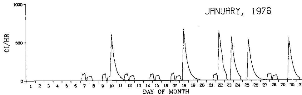
FIGURE 2c. Krypton-85 Release Rate for December, 1975 and January, 1976
