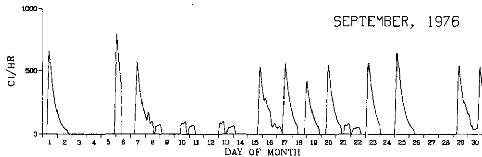
FIGURE 2g. Krypton-85 Release Rate for August and September, 1976
