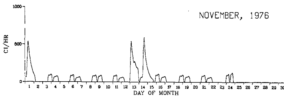
FIGURE 2h. Krypton-85 Release Rate for October and November, 1976
