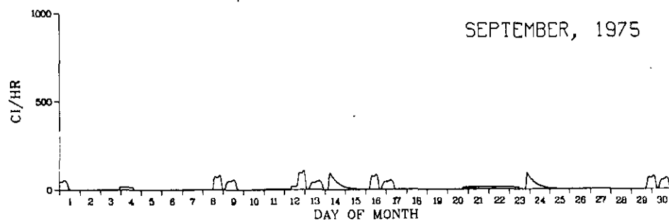
FIGURE 2a. Krypton-85 Release Rate for August and September, 1975
