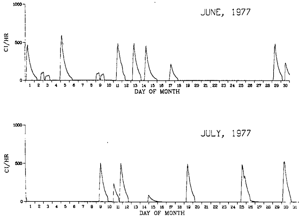
FIGURE 21. Krypton-85 Release Rate for June and July, 1977
