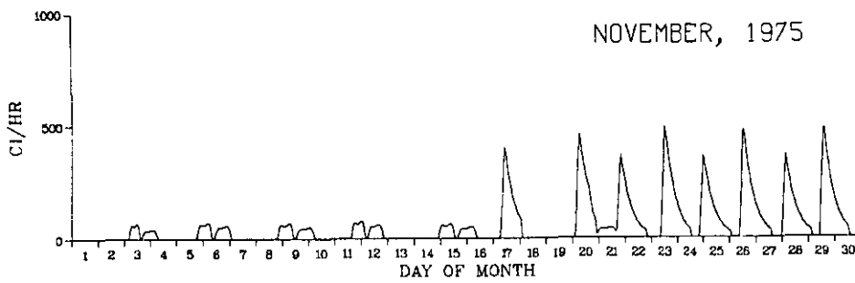
FIGURE 2b. Krypton-85 Release Rate for October and November, 1975
