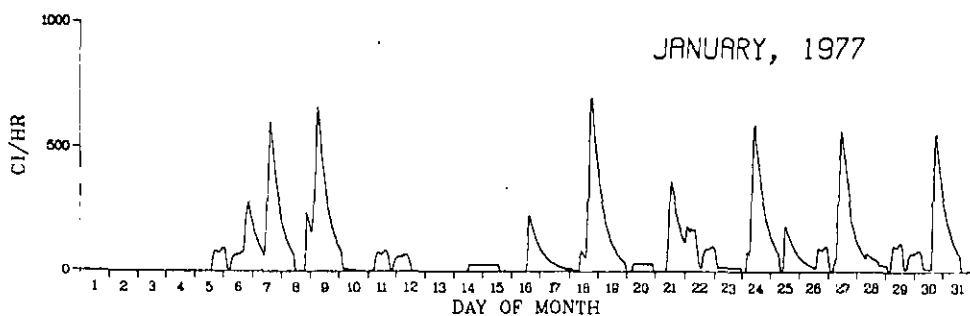
FIGURE 2i. Krypton-85 Release Rate for December, 1976 and January, 1977
