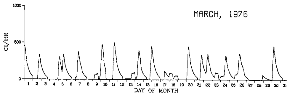
FIGURE 2d. Krypton-85 Release Rate for February and March, 1976
