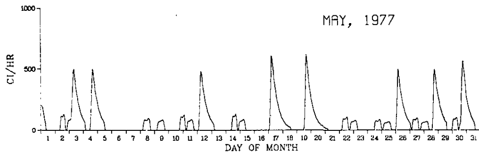
FIGURE 2k. Krypton-85 Release Rate for April and May, 1977
