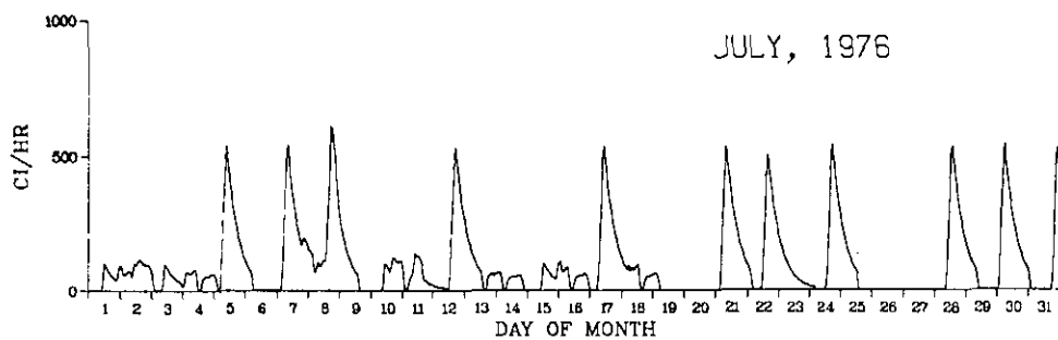
FIGURE 2f. Krypton-85 Release Rate for June and July, 1976
